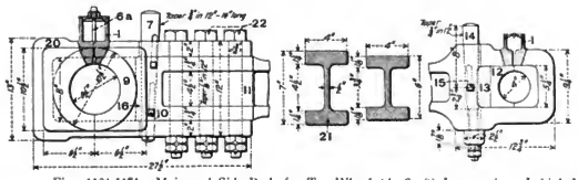
Figs. 1164-1171. Main and Side Rods for Ten-Wheel (4-6-0) Locomotive. Lehigh Valley.
